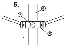
Fig 5. To adjust the height / angle arm (no.6) Loosen the screw part no.7, use the winder to project the fabric (adjustment bar part no.8 will move accordingly) Once the height is set tighten up screw, part no.7.
