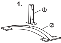
Fig 1. Assemble and connect part 1 & 2 together using M10 x 40mm bolts. This will form part of a leg (base for awning) Repeat process to form the other leg.
