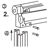
Fig 2. Insert roller part 3 over the top of the upright post (mid section no.4) connect both parts together using M8 x 60mm bolts Repeat same process and connect the other side.
