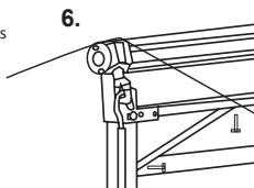
Fig 6. Use screw M8 x 50mm bolt and M8 x 35mm to install the slanted bars on both sides. The awning is now assembled and ready to use.
