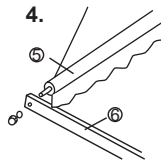
Fig 4. Connect the angle bar (no.6, left and right) onto the end of the front bar part no.5. Repeat same process to connect the opposite side.
