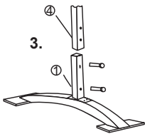
Fig 3. Two people will be required to complete this step. Connect the mid sections (no.4) with the upright legs, (left/right) by using M8 x 50mm bolts. Do not attempt to lift this unit onto legs without assistance.
